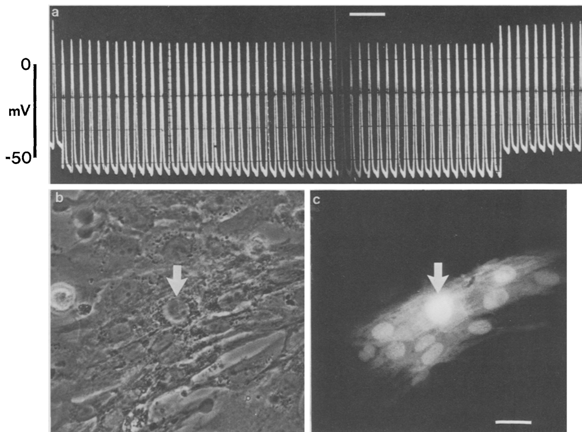
Fig. 7. Dye transfer from an injected muscle cell to neighboring cells during exposure to A23187. (a-c): Cell injected after a 10-min exposure to 25\ \mu\text{M} A23187 and not fixed. Note that dye transfer has occurred to neighboring muscle cells but not to neighboring fibroblasts. Arrows indicate the injected cell nucleus. Calibration bar in a represents 3 sec. Calibration for b and c = 24\ \mu\text{m}
