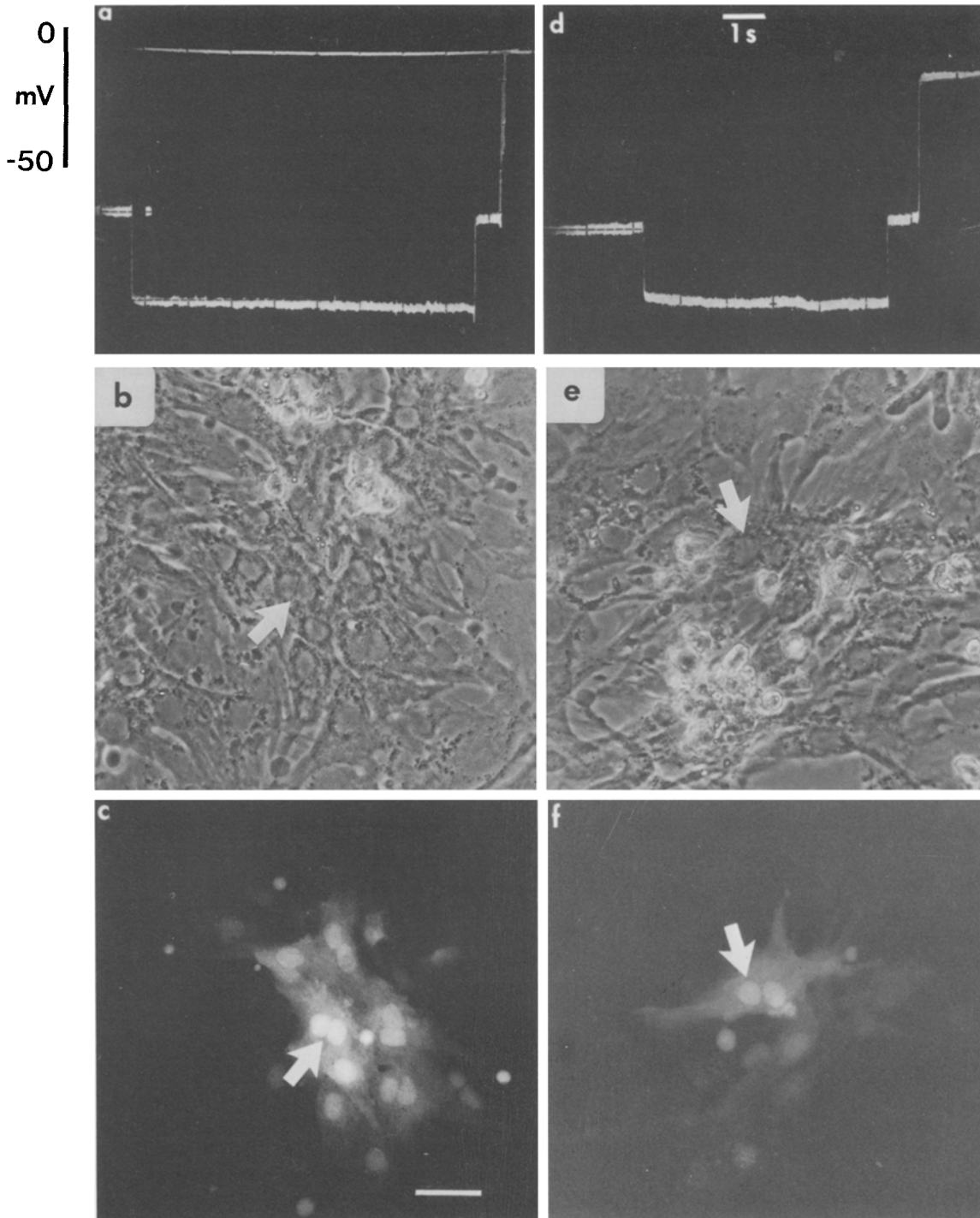
Fig. 6. Dye transfer from an injected muscle cell to neighboring cells during exposure to monensin. ( a-c ): Cell injected for 17 sec after 5 min in 25 \mu M monensin and immediately fixed. ( d-f ): Cell injected for 11 sec after 22 min in 25 \mu M monensin and immediately fixed. Note in both cases that dye transfer occurred. Arrows indicate the injected cells; calibration bar for all micrographs = 24 \mu M. Time calibration for a : equivalent bar length to that seen in d (1 sec) would equal 2.4 sec
